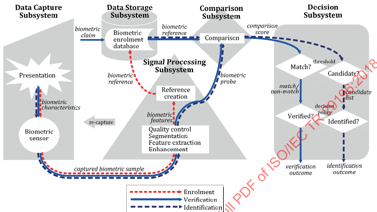
Figure 1 — Components of general biometric system
