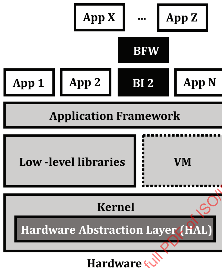
Figure 5 — Illustration on how the ISO/IEC 30106 Framework (BFW) may be implemented at application level
