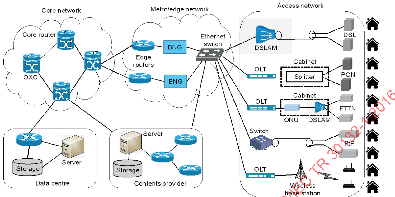
Figure 1 — High-level network structure for the Internet [23]
