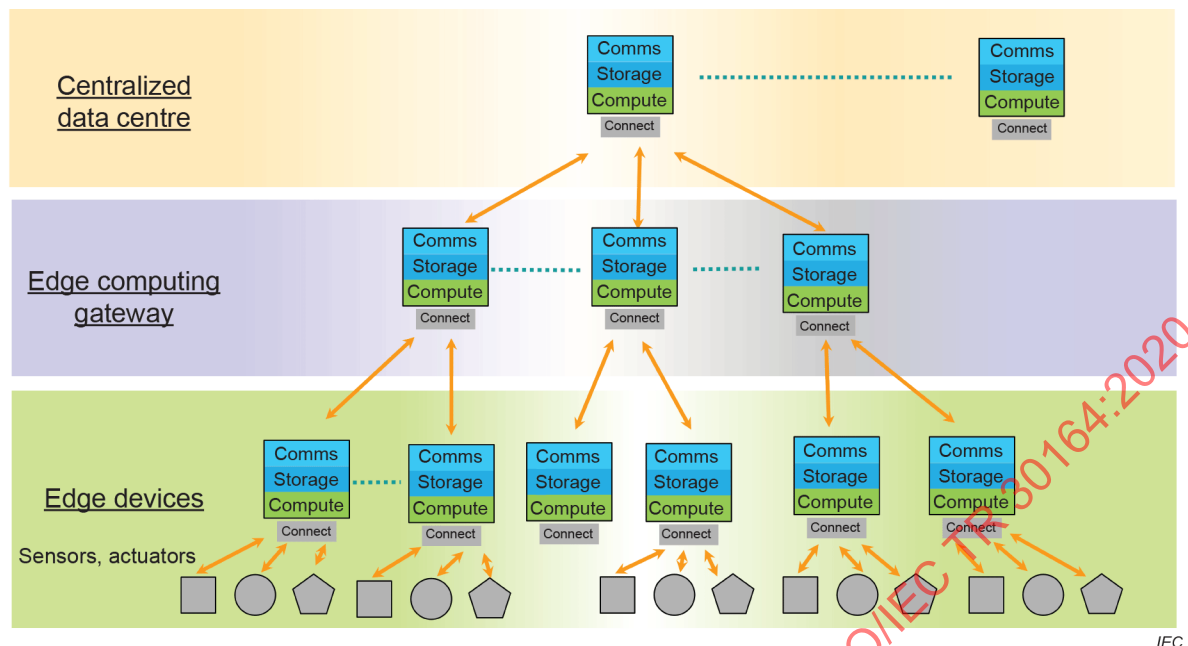
Figure 5 – Edge computing three-tier deployment model
