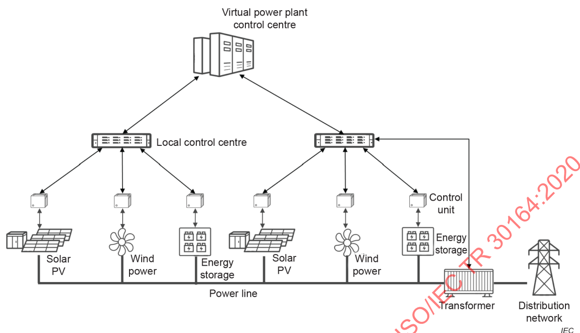
Figure 11 – Concept of centralized monitoring of power plants
