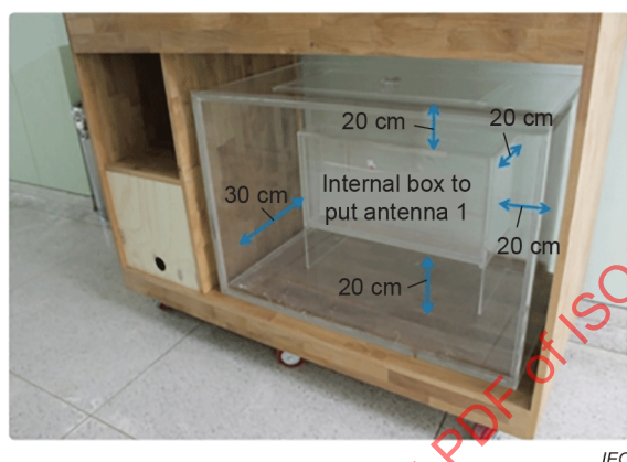
Figure 21 – Experimental water tank for comparing magnetic field communication characteristics according to medium and distance
