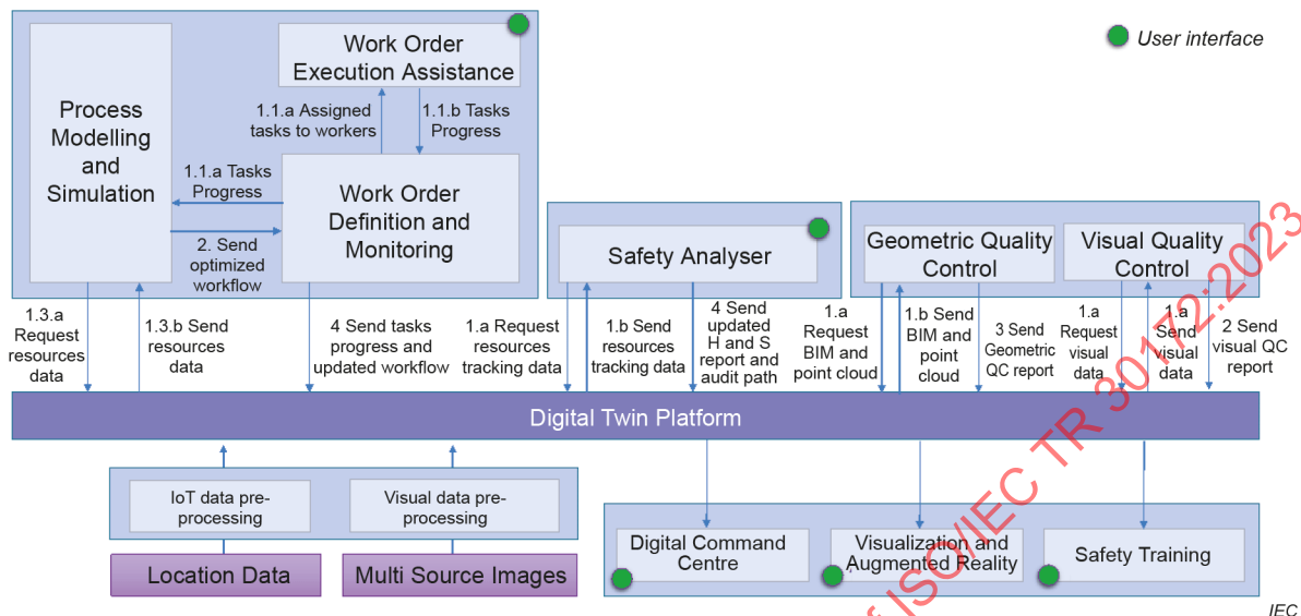
Figure B.8 – Use case diagram: during construction
