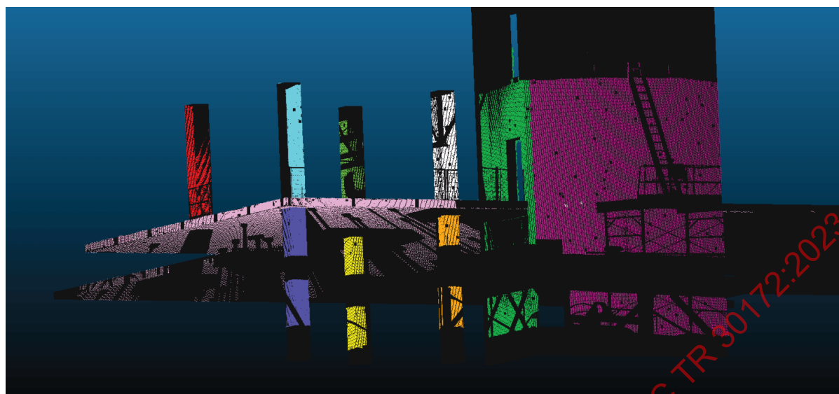
Figure B.4 – Segmented construction components after voxel space point matching
