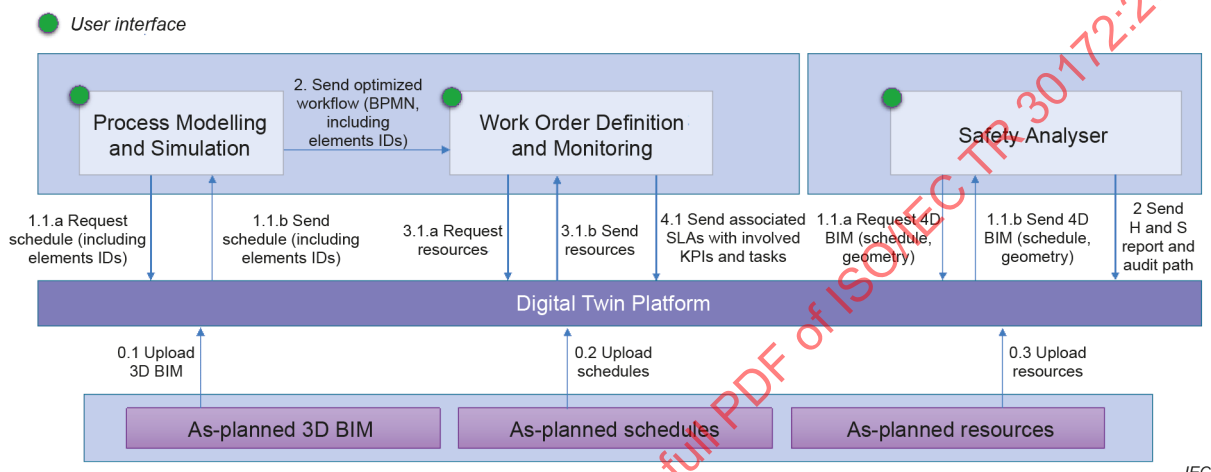
Figure B.7 – Use case diagram: before construction starts
