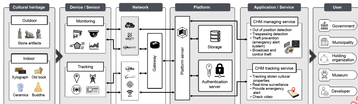
Figure 3 – System model for IoT-based management of cultural heritage
