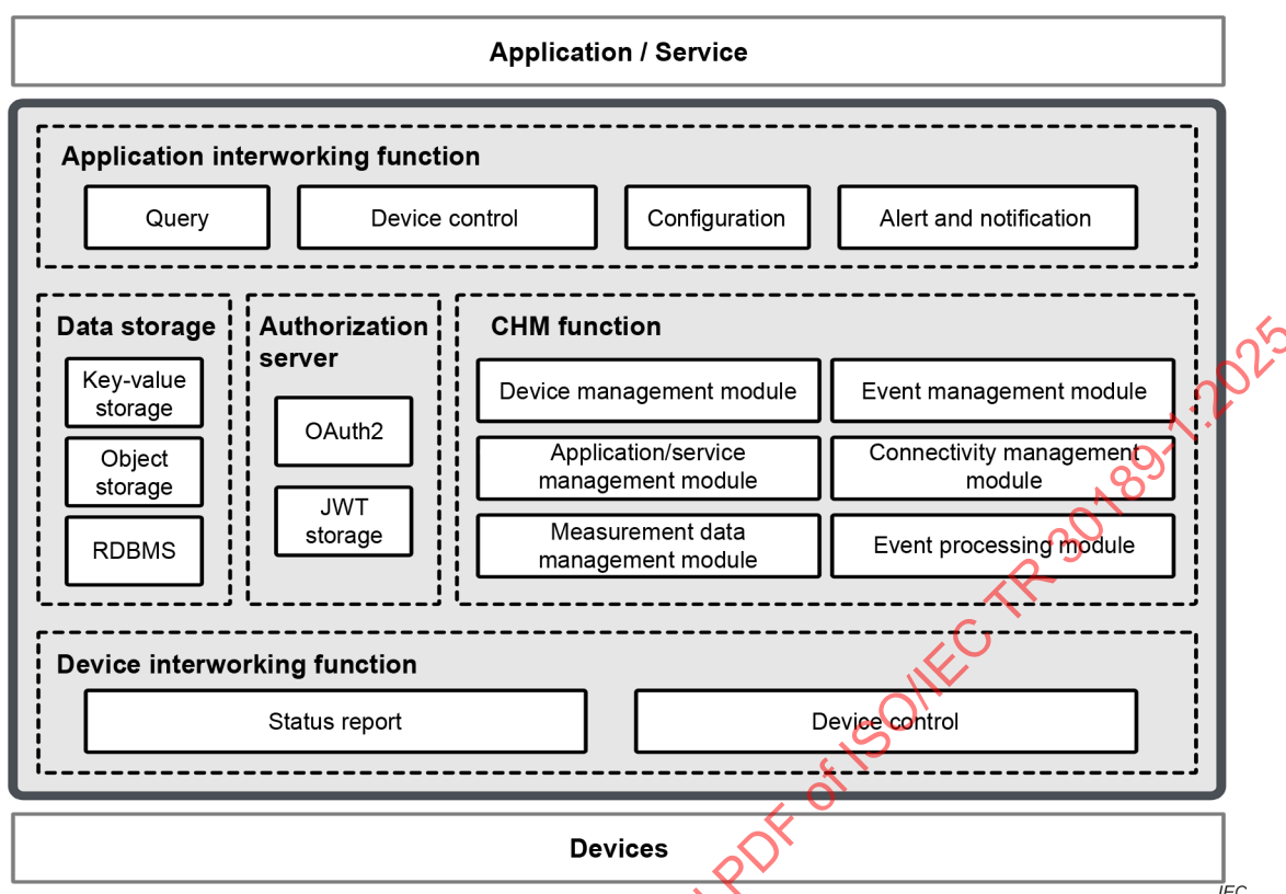
Figure 4 – Platform functions for IoT-based CHM
