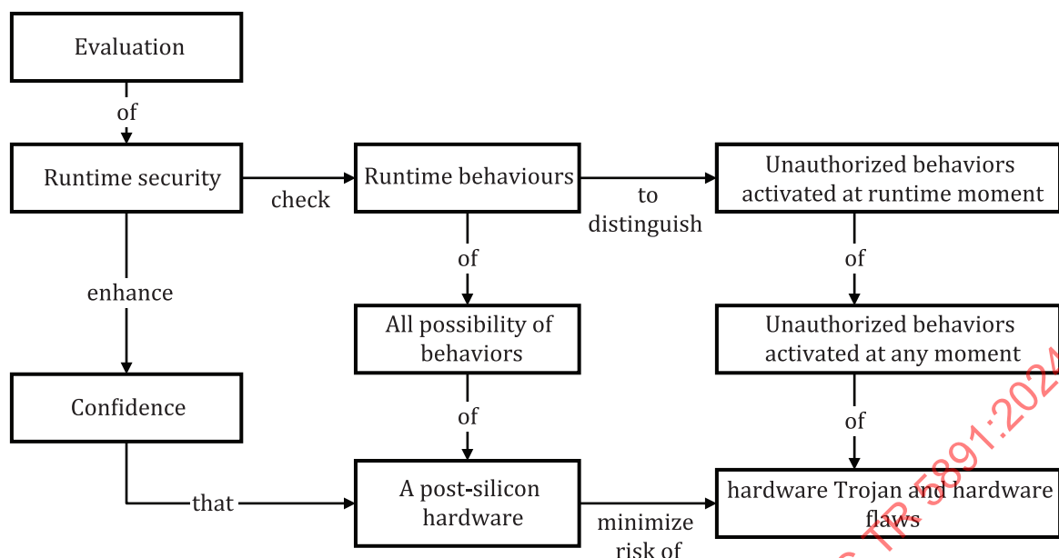
Figure 2 — Runtime hardware-behaviour-based security — concepts and relationships
