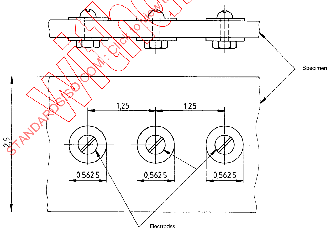
Figure B.1 — Application of binding-post electrodes to flat, solid specimens
