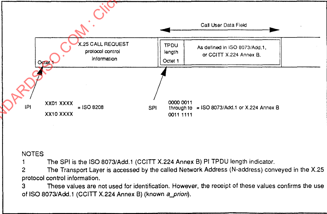
Figure A.2 - IPI and SPI when ISO 8073/Add.1 (CCITT X.224 Annex B) is operated over ISO 8208
