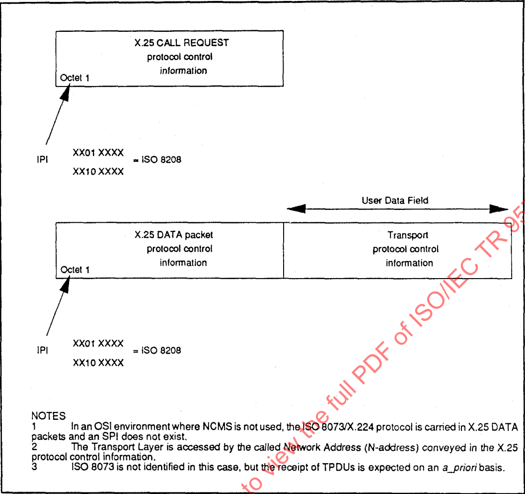
Figure A.3 - Location of IPI and SPI when ISO 8073 is used over ISO 8208
