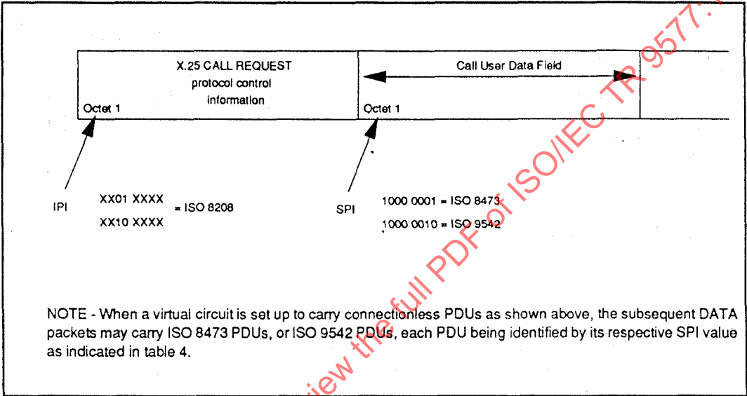
Figure A.1 - IPI and SPI when ISO 8473 or ISO 9542 is operated over ISO 8208
