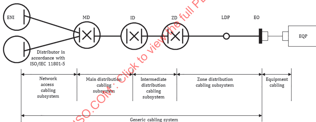
Figure 5 — Data centre cabling subsystems according to ISO/IEC 11801-5
