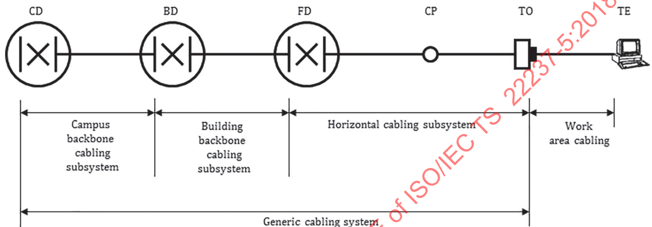
Figure 6 — Office cabling subsystems according to ISO/IEC 11801-2
