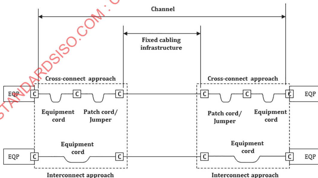
Figure 9 — Transmission channels (interconnect and cross-connect)
