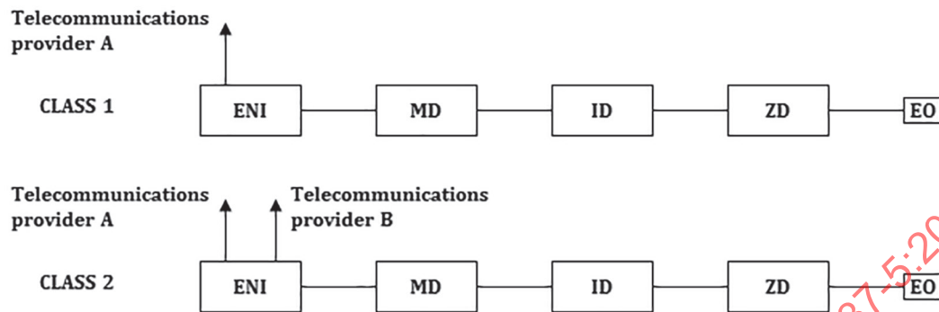
Figure 10 — ENI redundancy for Class 1 and 2
