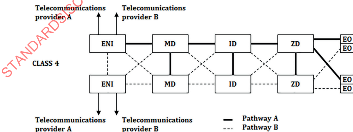
Figure 13 — Redundant multipath telecommunication cabling Class 4
