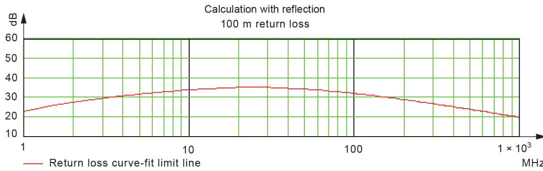
Figure 8 – 100 m cable return loss with a reflection of 0,03 at both ends (6 \Omega mismatch, ~23 dB return loss at 1 MHz)
