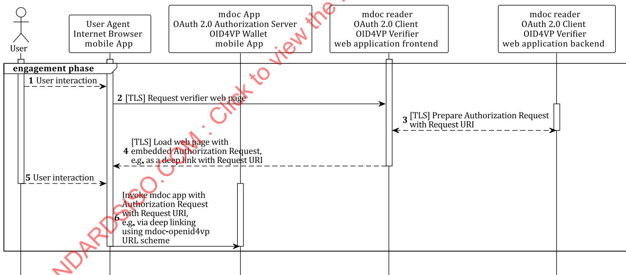
Figure B.1 — Engagement phase sequence diagram
