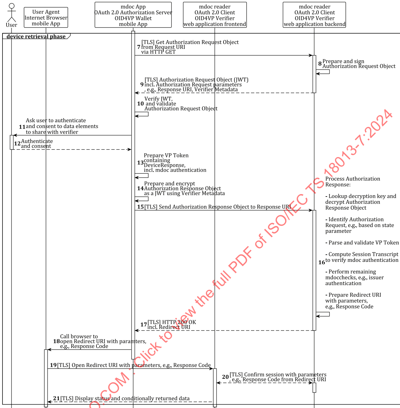
Figure B.2 — Device retrieval phase sequence diagram
