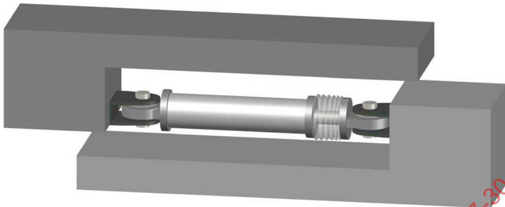
Figure 3 — Oil damper
