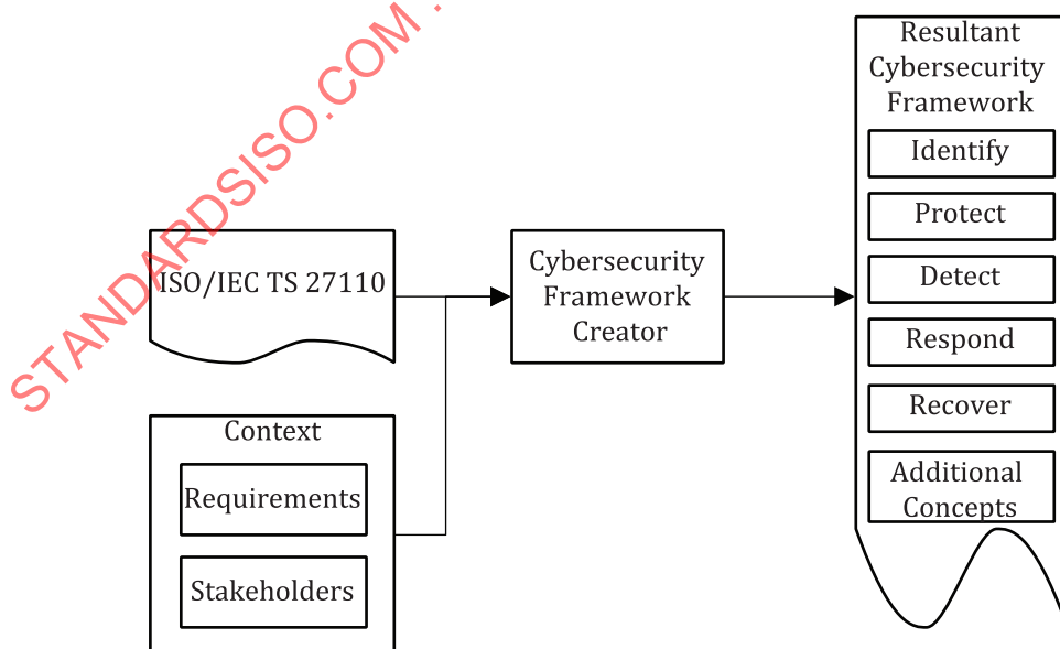
Figure 1 — Creating a cybersecurity framework using ISO/IEC TS 27110
