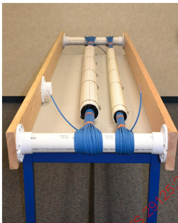
Figure F.4 – Test set-up for cable bundles in conduit
