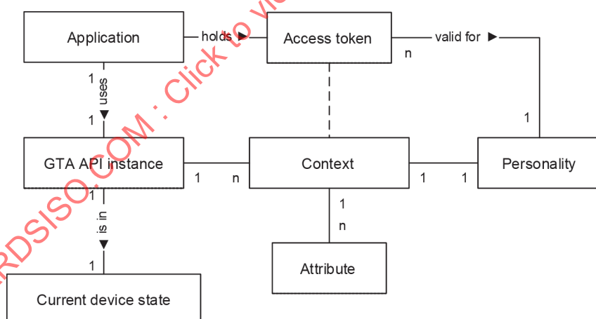
Figure 8 – Object information model (runtime view)
