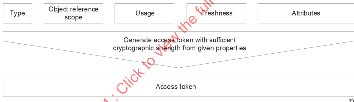
Figure 14 – Access token
