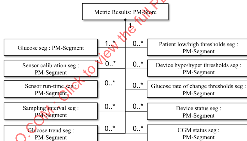
Figure 3—CGM persistent store model example
