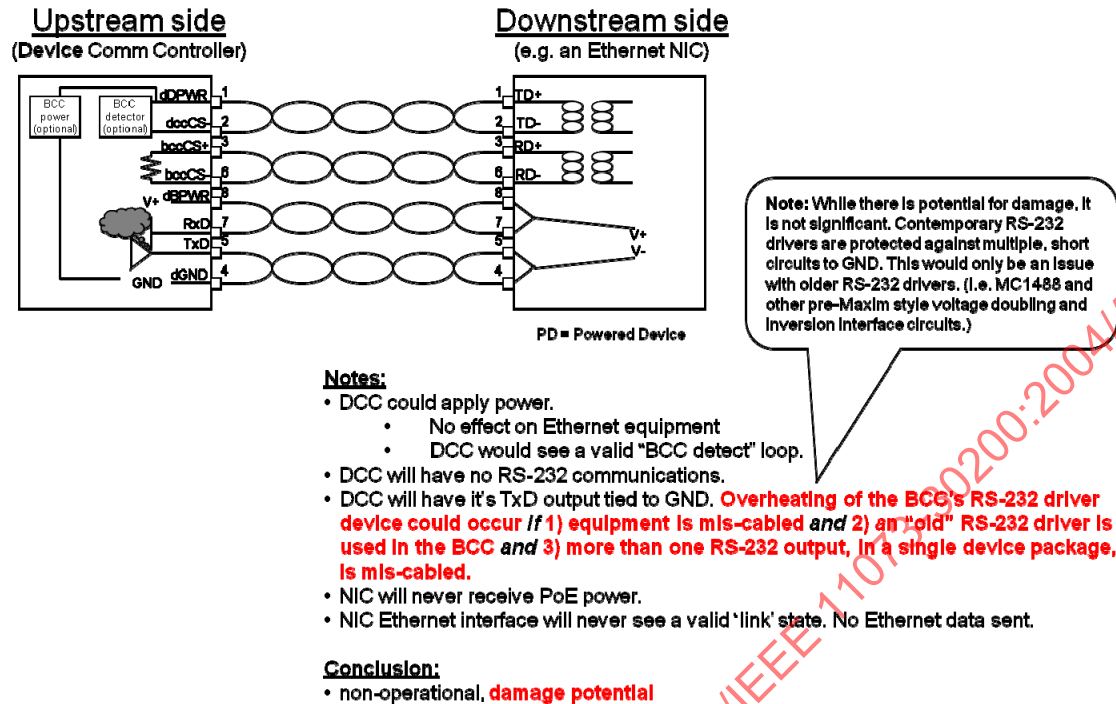
Figure O.17—Scenario 12: Upstream—30200: DCC/downstream—PoE: alternative B
