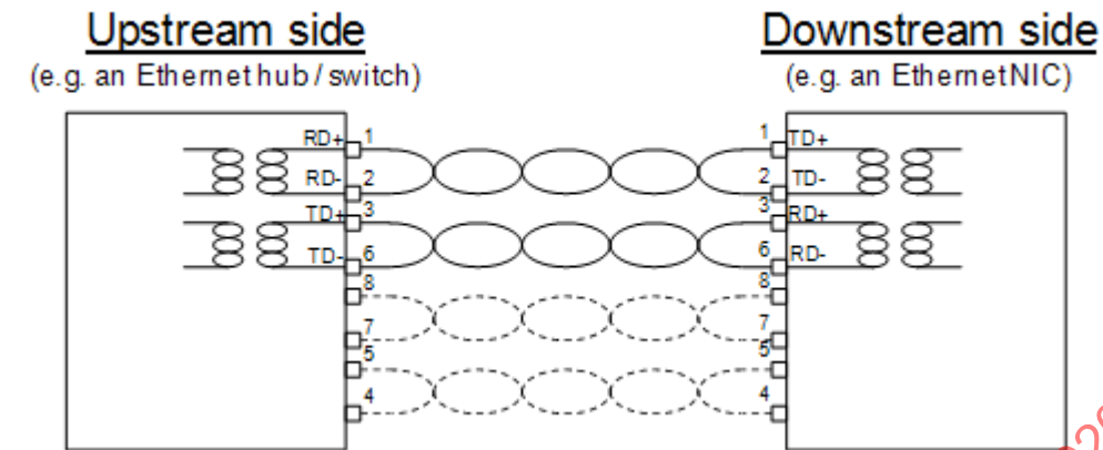
Figure O.3—Intended use: Ethernet
