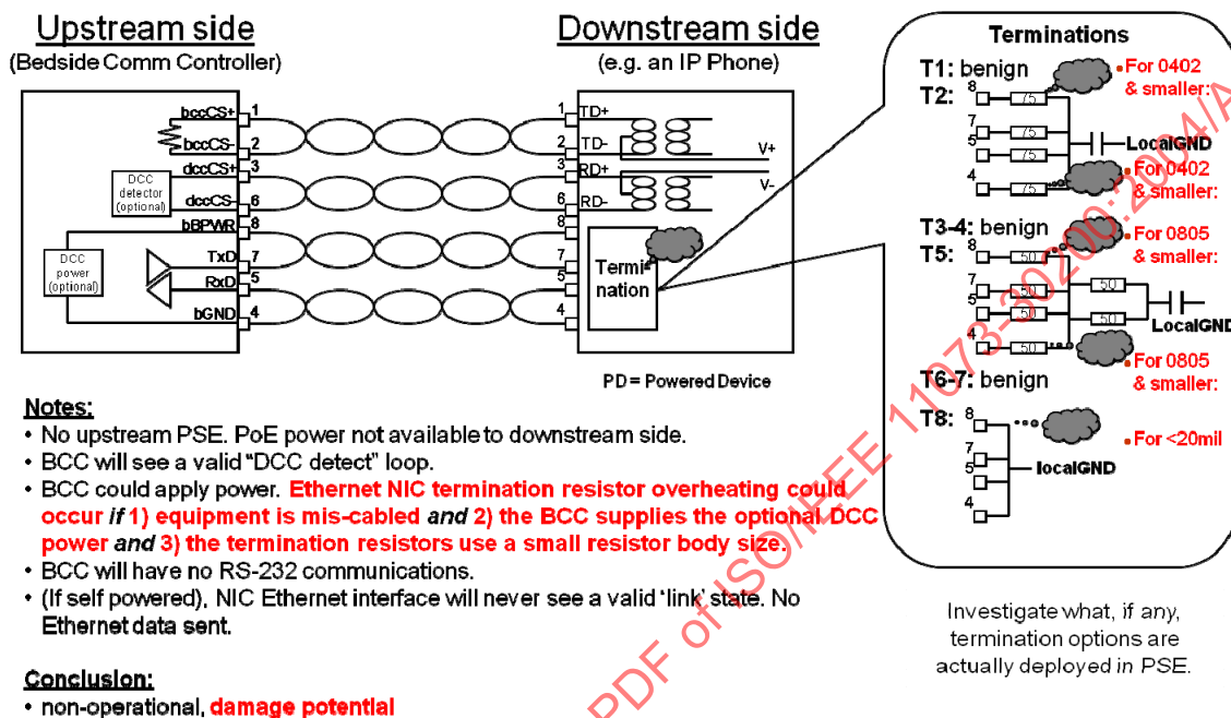
Figure O.13—Scenario 8: Upstream—30200: BCC/downstream—PoE: alternative A
