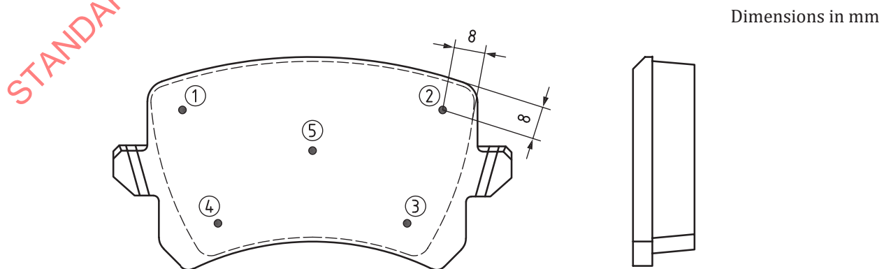
Figure 3 — Position of thickness measurement points
