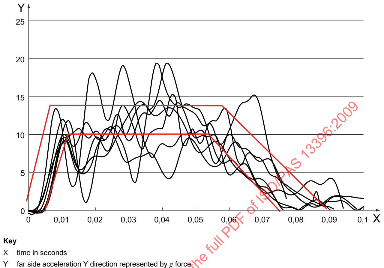
Figure 3 — General requirements for sled acceleration
