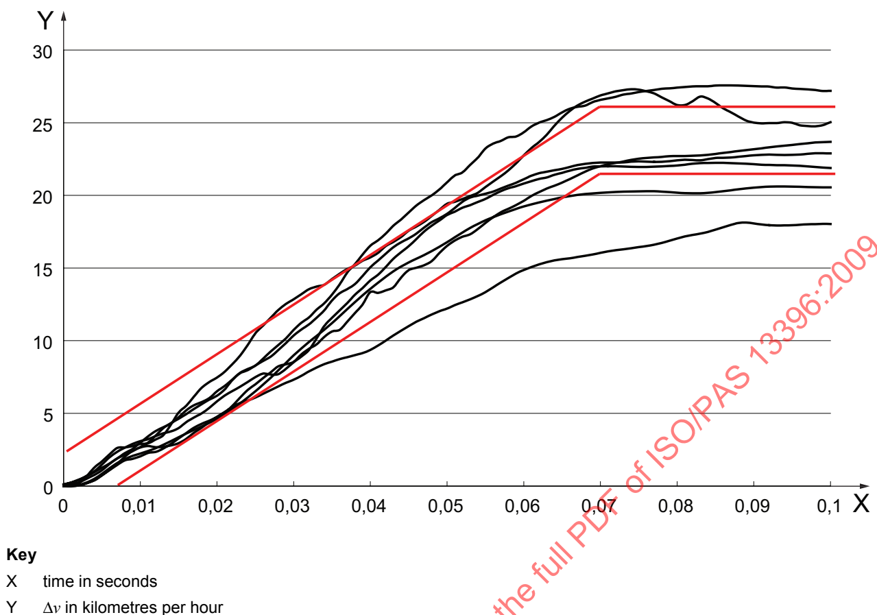
Figure 4 — General requirements for sled \Delta v
