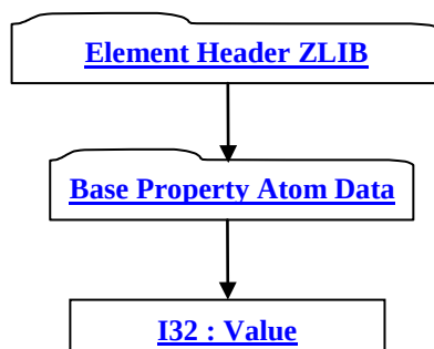
Figure 69: Integer Property Atom Element data collection
