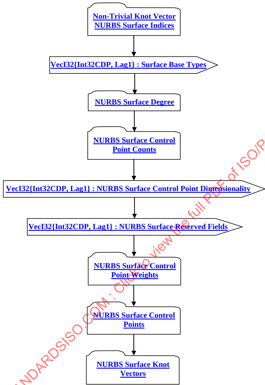
Figure 115: Surfaces Geometric Data data collection
