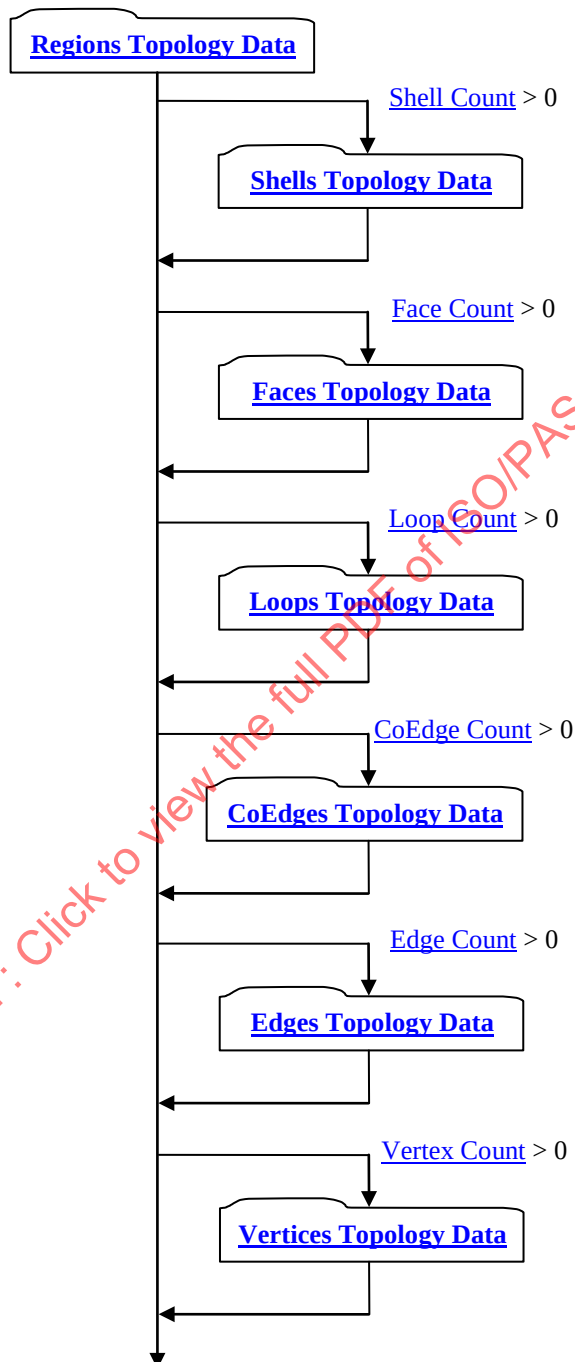
Figure 105: Topology Data data collection
