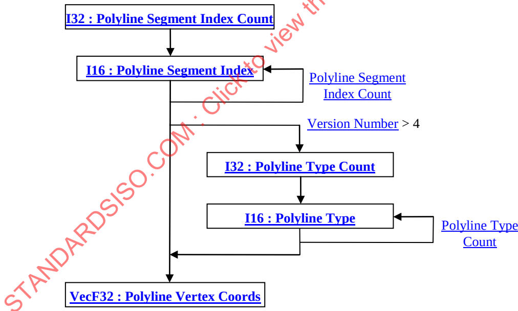
Figure 146: Non-Text Polyline Data data collection
