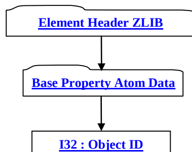
Figure 71: JT Object Reference Property Atom Element data collection
