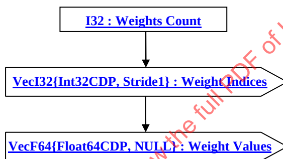
Figure 187: Compressed Control Point Weights Data data collection
