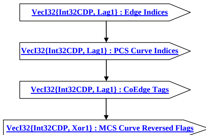
Figure 111: CoEdges Topology Data data collection
