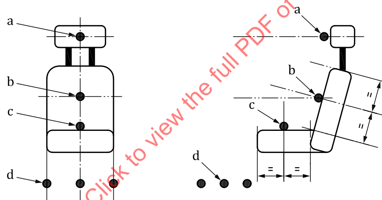
Figure 4 — Emission validation positions for area 4
