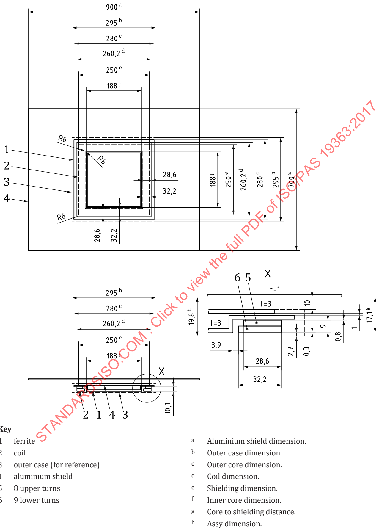
Figure A.1 — Mechanical dimensions of the MF-WPT1/Z1 circular reference EV device
