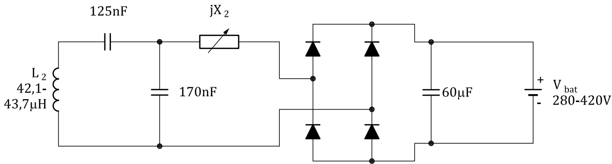
Figure C.4 — Schematics of power electronics for the MF-WPT2/Z2 circular reference EV device
