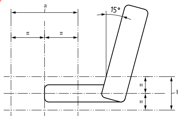
Figure 5 — Seat position adjustment
