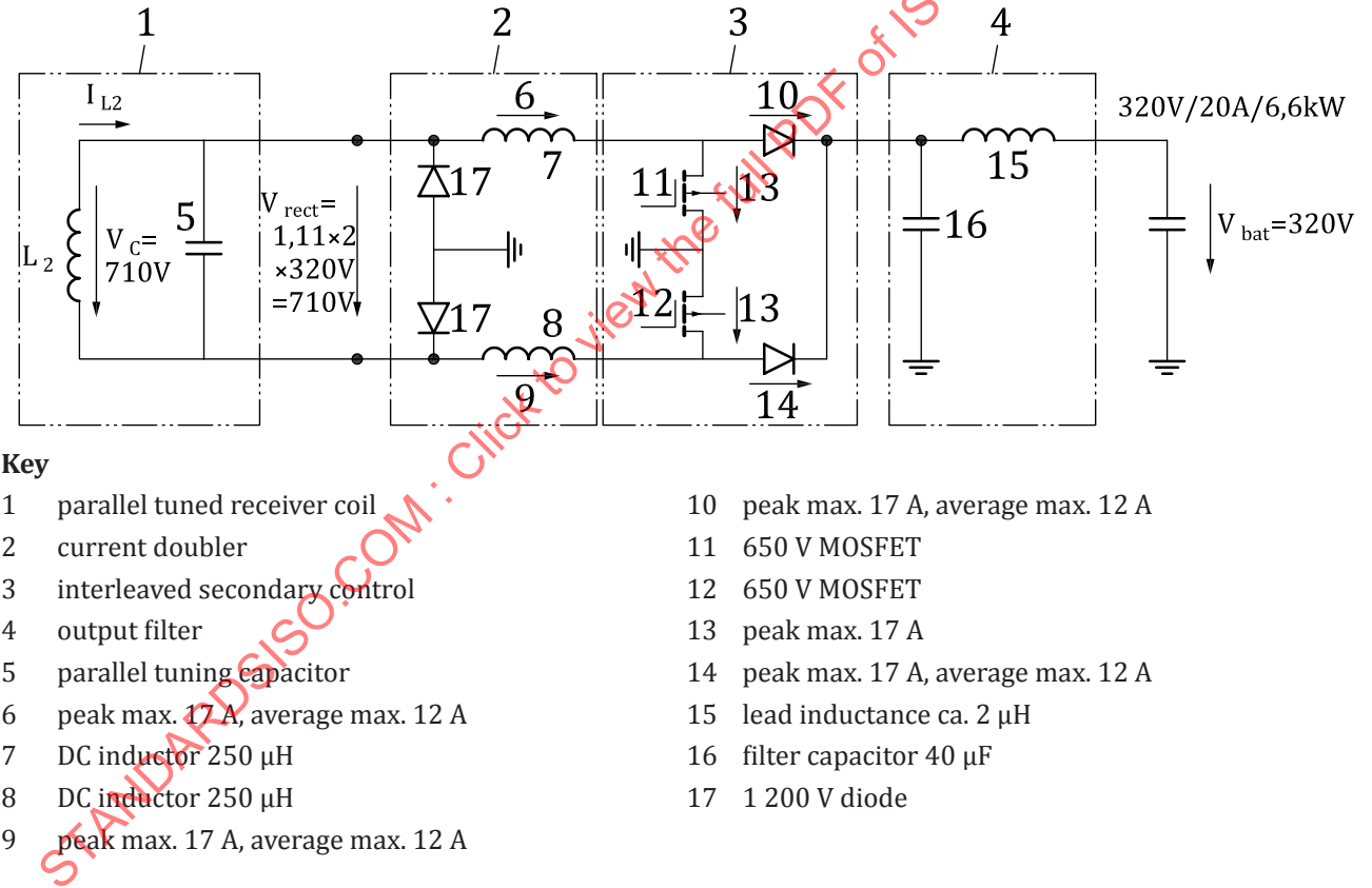
Figure D.6 — Schematics of power electronics for the MF-WPT2/Z2 DD reference EV device
