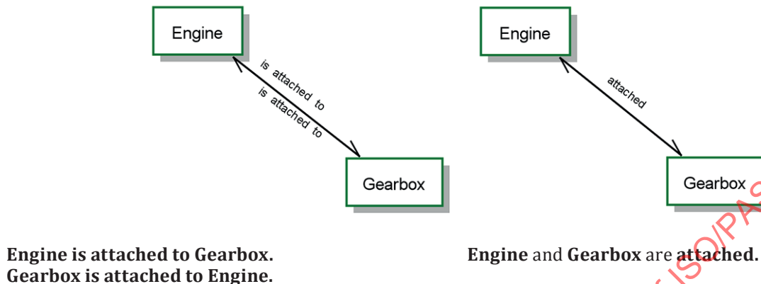
Figure 15 — Bidirectional (left) and its equivalent reciprocal tagged structural link (right)
