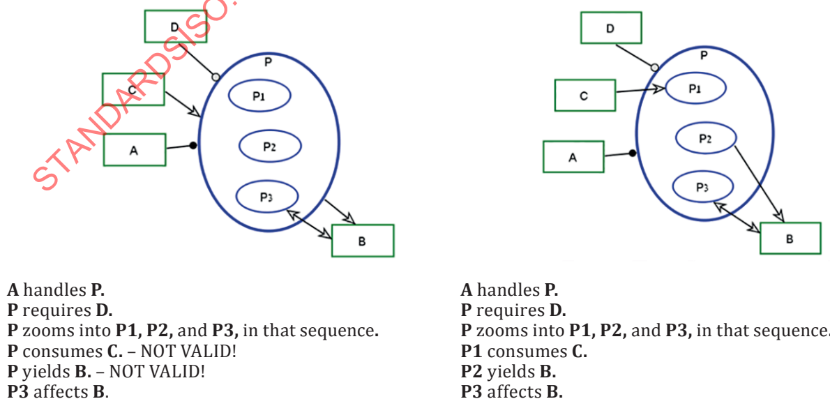
Figure 51 — Link distribution restriction for consumption and result links
