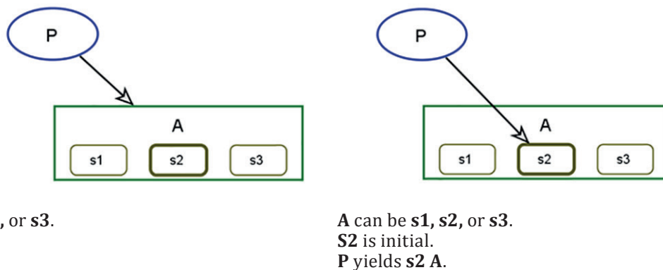
Figure 10 — Correct (left) and incorrect (right) result link to an object with an initial state
