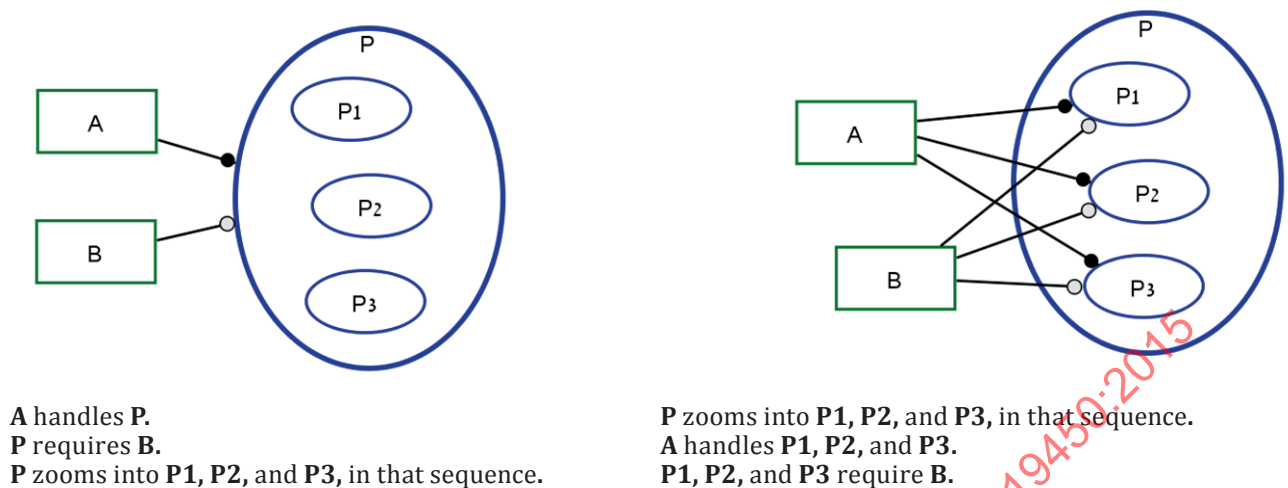
Figure 50 — In-zooming link distribution
