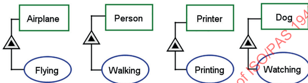
Figure 20 — Object attribute examples
