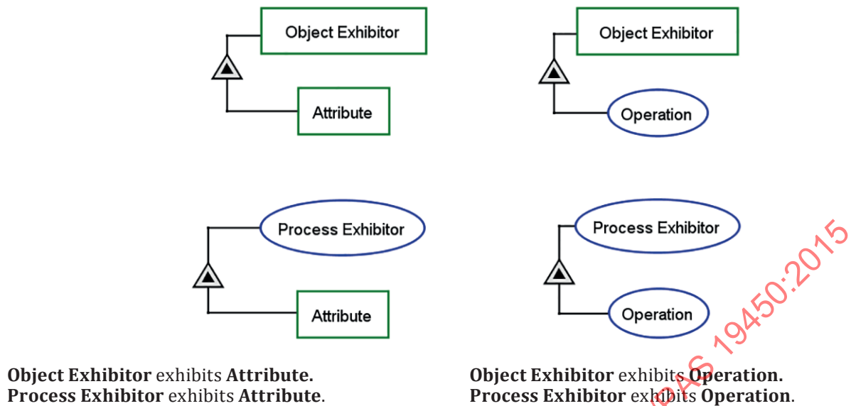
Figure 19 — The four exhibition-characterization feature combinations
