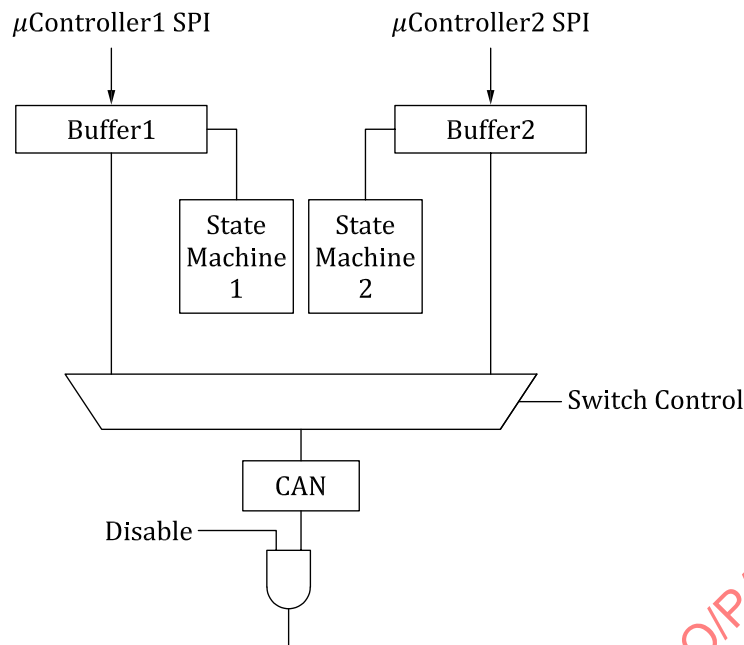
Figure 14 — PLD architecture
