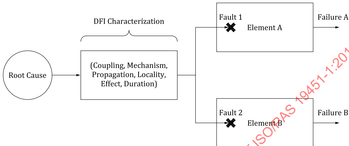
Figure 21 — Dependent failure root cause
