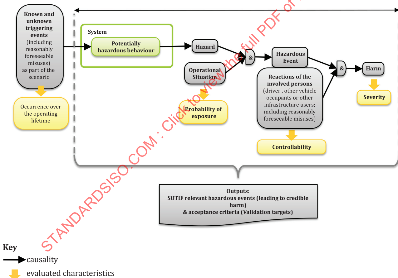
Figure 12 — An illustration of common elements of hazard analysis in the ISO 26262 series and in this document
