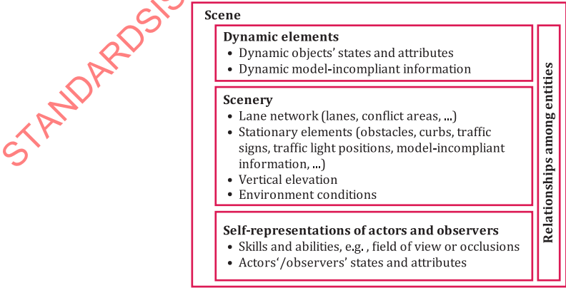
Figure 4 — Characteristics of a scene
