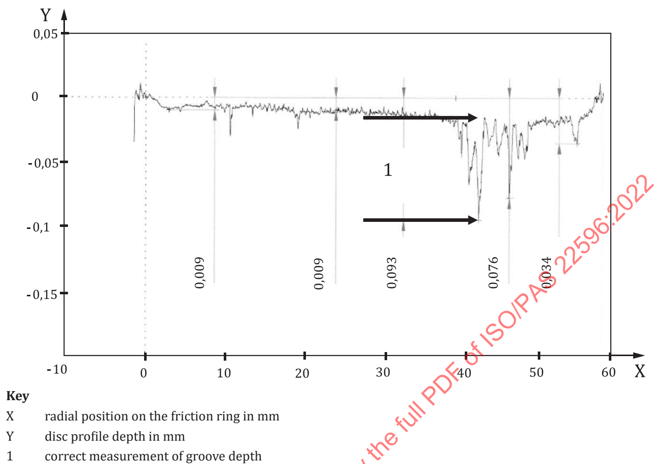
Figure 7 — Example for disc surface profile measured radially with measurement of groove depth for the test report
