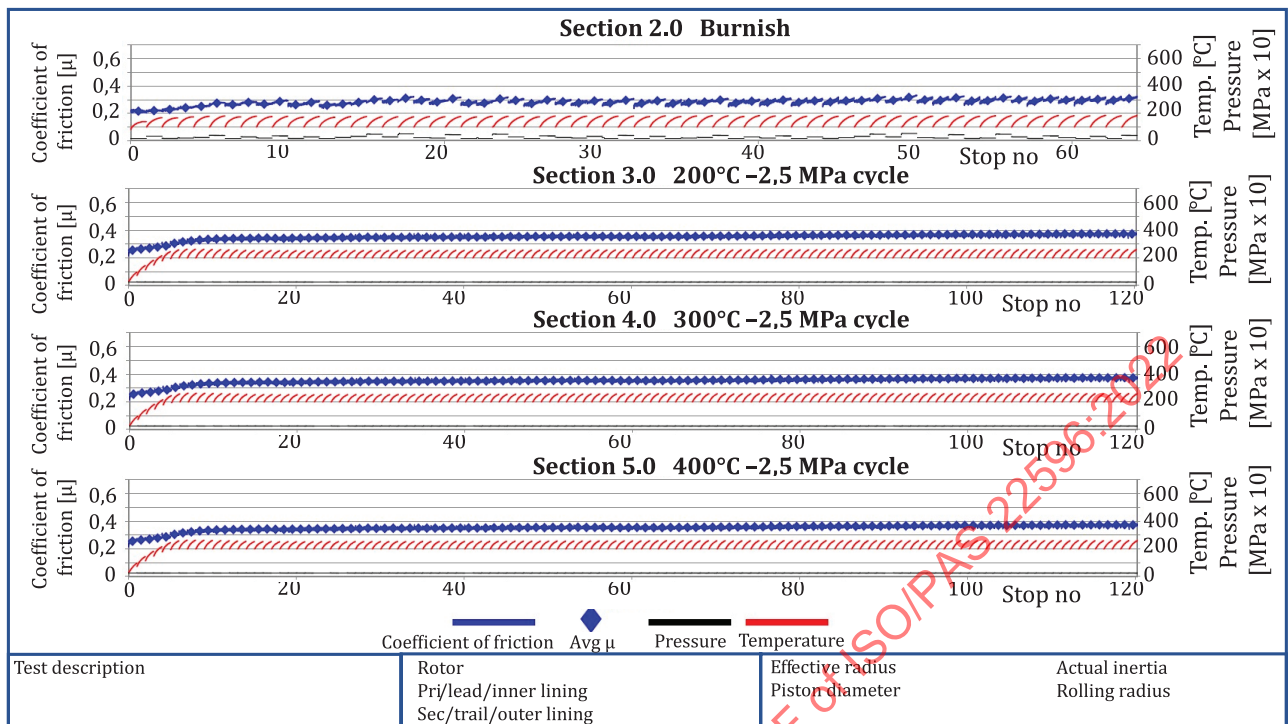
Figure B.4 — Proposal for general MPU test report — “burnish data plot”
