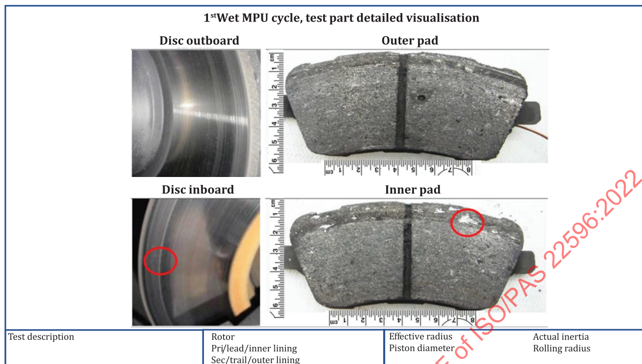
Figure B.6 — Proposal for the MPU test report — “detailed visualization of disc and pads”
