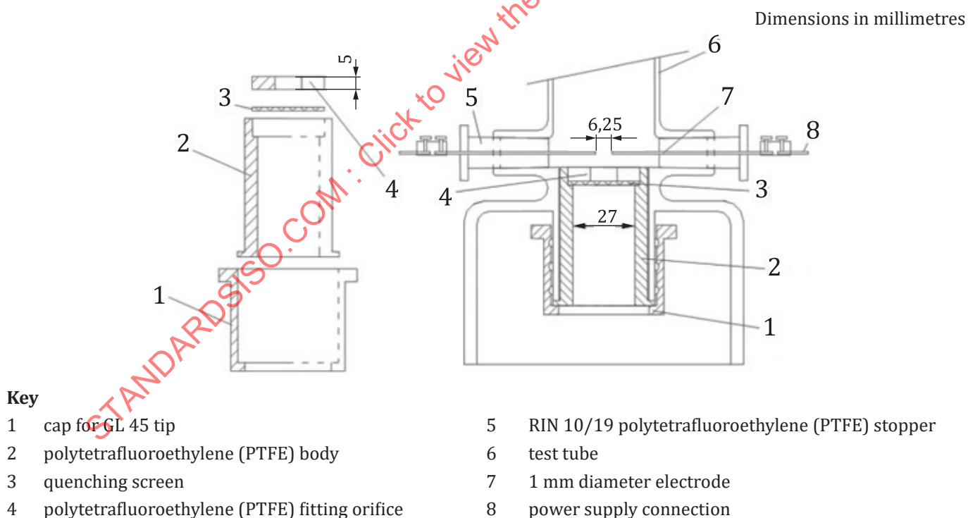
Figure 4 — Drawing of the lower end of the tube showing the ignition electrodes and the damping (fitting) orifice
