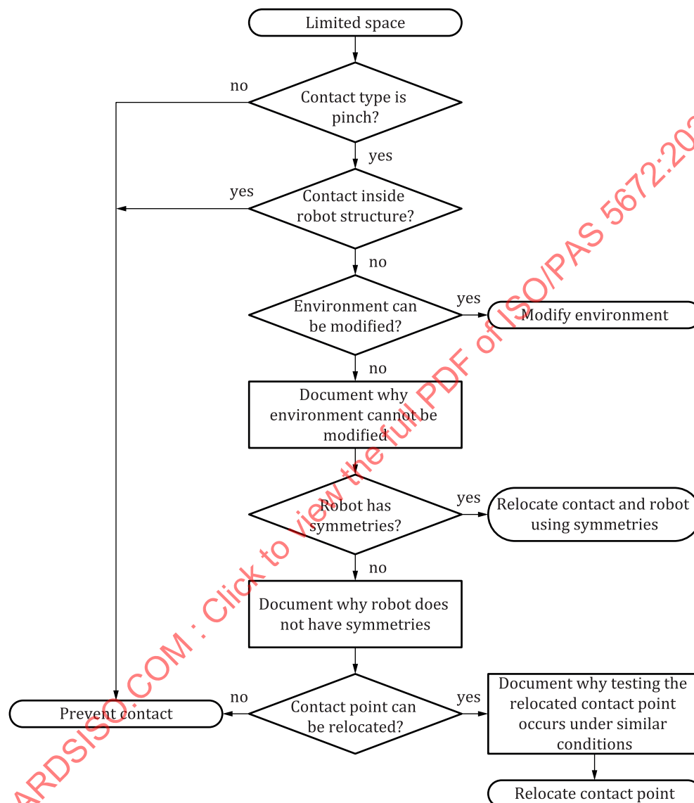
Figure 6 — Procedure to follow when a PFMD cannot be installed at the testing point due to limited space.
