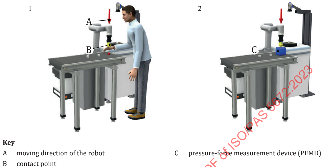
Figure C.2 — Example 1 “Pick-and-Place Application”: Contact hazard 1 (pinch of the hand when robot approaches workpiece on the conveyer)
