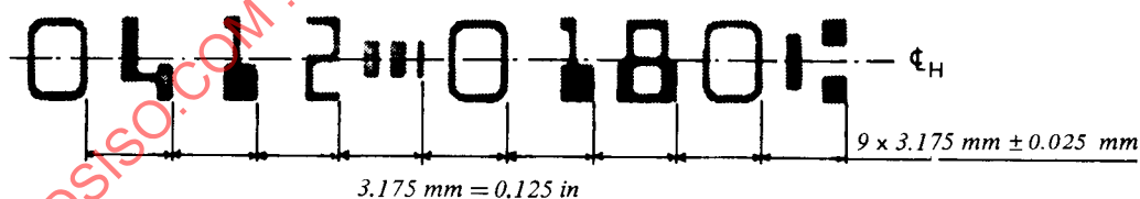
FIG. 16 - Distance between characters
