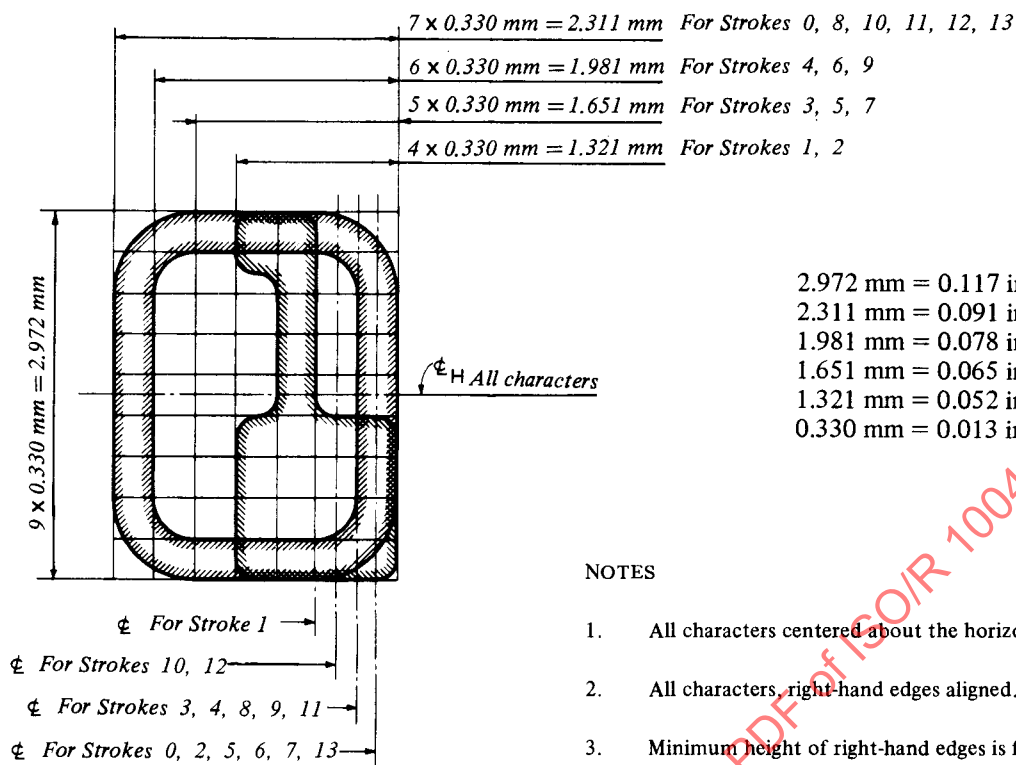
FIG. 15 - Character design matrix. This is a 7 x 9 matrix of 0.330 mm (0.013 in) squares
