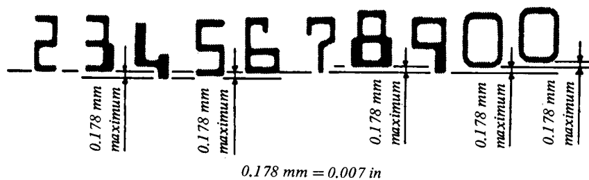
FIG. 17 - Allowable variation in vertical alignment
