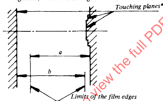
FIG. 3 — Position of film edges relative to camera-barrel touching planes
