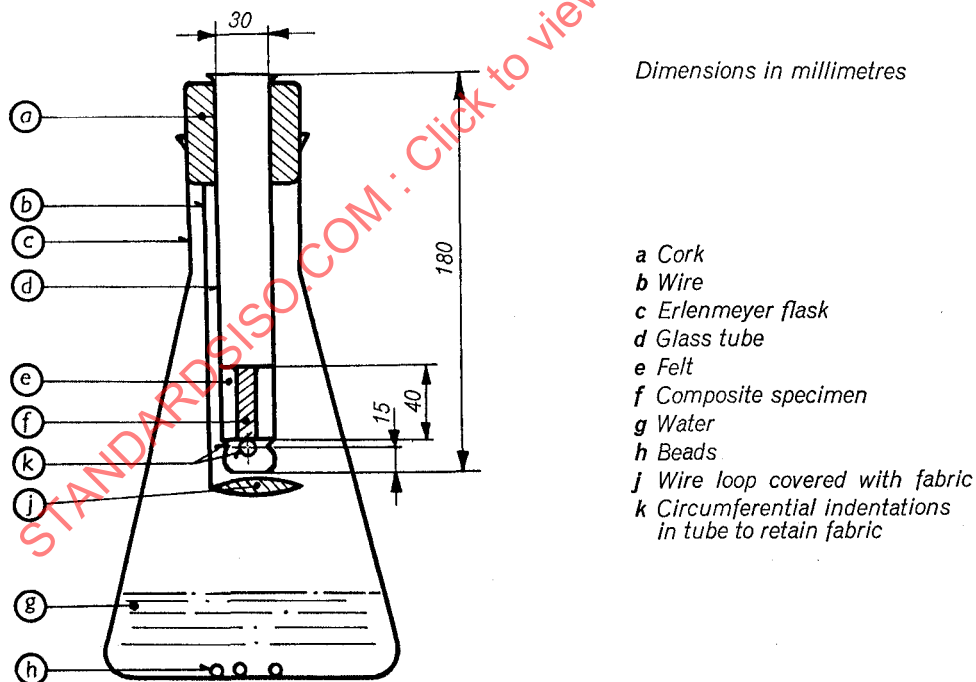
FIGURE.— Apparatus for colour-fastness to steaming
