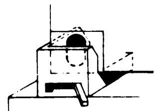
View "C" Example of deck securing fitting which provides gathering plus both horizontal and vertical restraint
