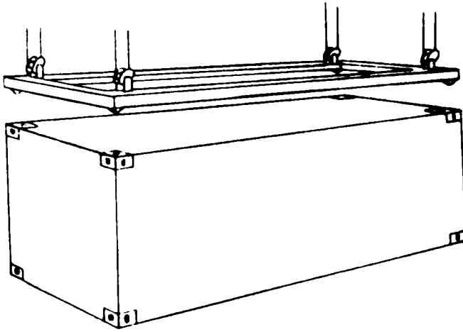
(a) Top lift automatic by means of spreader twist locks
