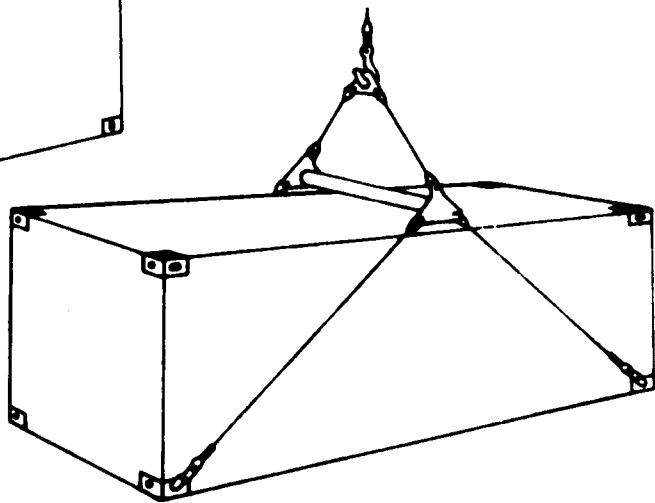
(d) Bottom lift by means of slings
