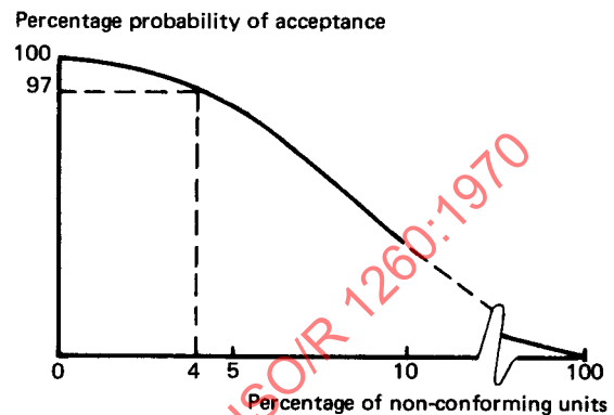
FIG. 1 — Operating characteristic (OC) curve
