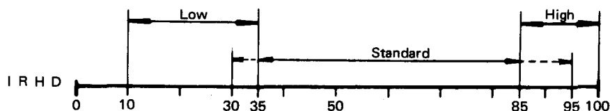
FIG. 1 – Range of applicability of hardness tests
