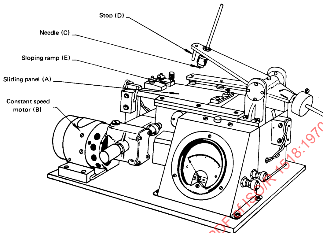
FIG. 2 — Suitable type of mechanized scratch test apparatus
