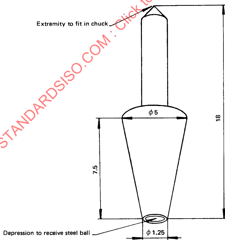
FIG. 3 — Suitable shank for scratch test needle
