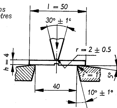
FIG. 6.—Striking edge and anvil for standard small bar without and with notch
