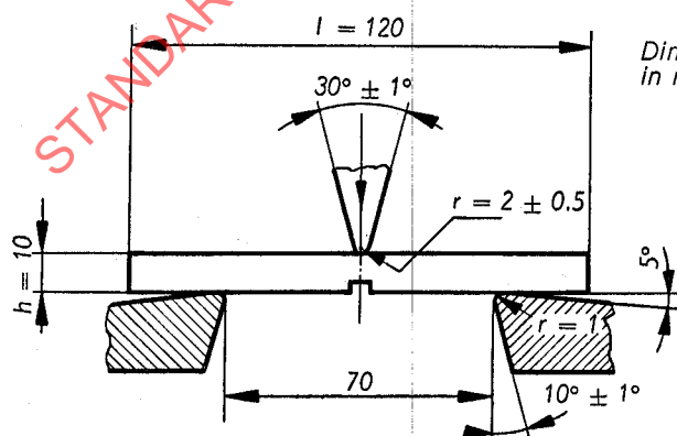
FIG. 5.—Striking edge and anvil for standard bar without and with notch
