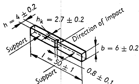
FIG. 2.—Standard small bar with notch
