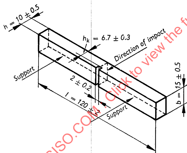
FIG. 1.—Standard bar with notch
