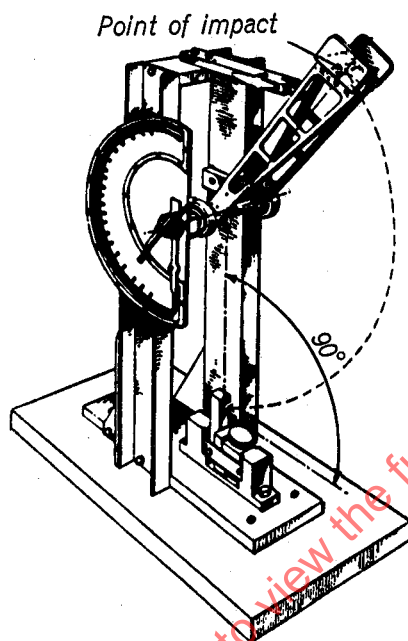
Fig. 1.—Cantilever beam (Izod Type) impact machine
