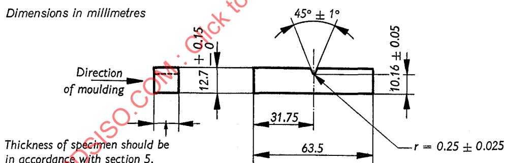
Fig. 2.—Specimen for Cantilever beam (Izod Type) impact machine
