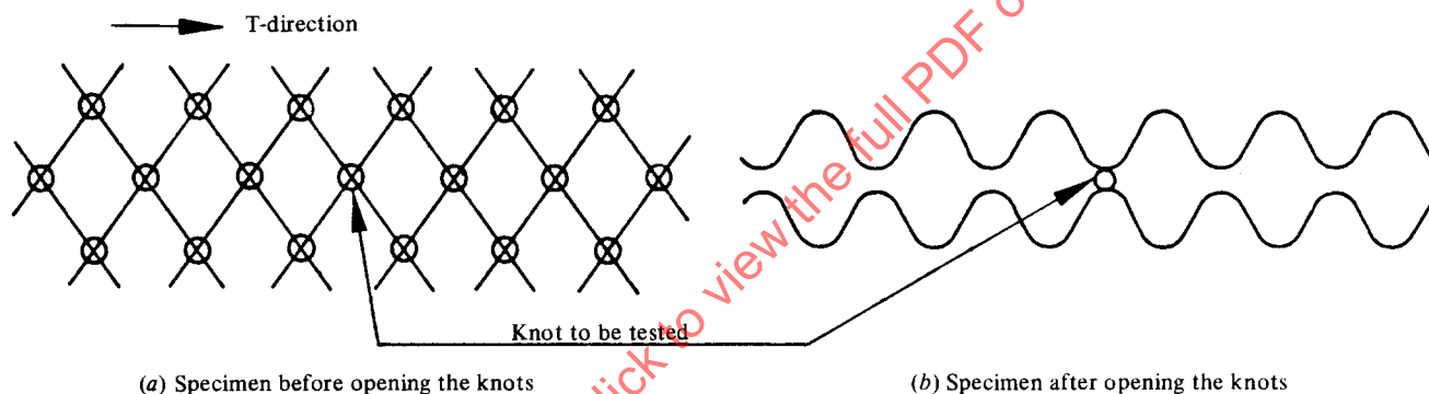
FIG. 3 — Preparation of specimen for determination of knot breaking load
