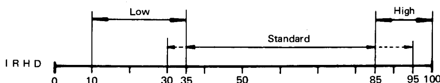
FIG. 1 – Range of applicability of hardness tests
