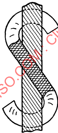
Fig. 1 S twist
