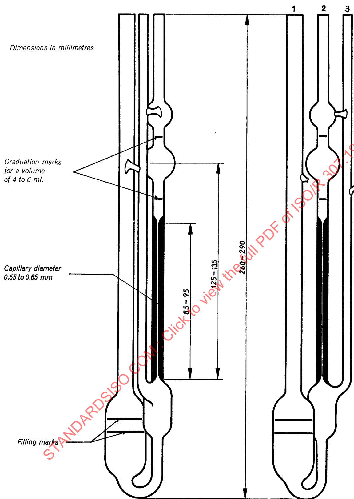
FIGURE—Ubbelohde Viscometer
