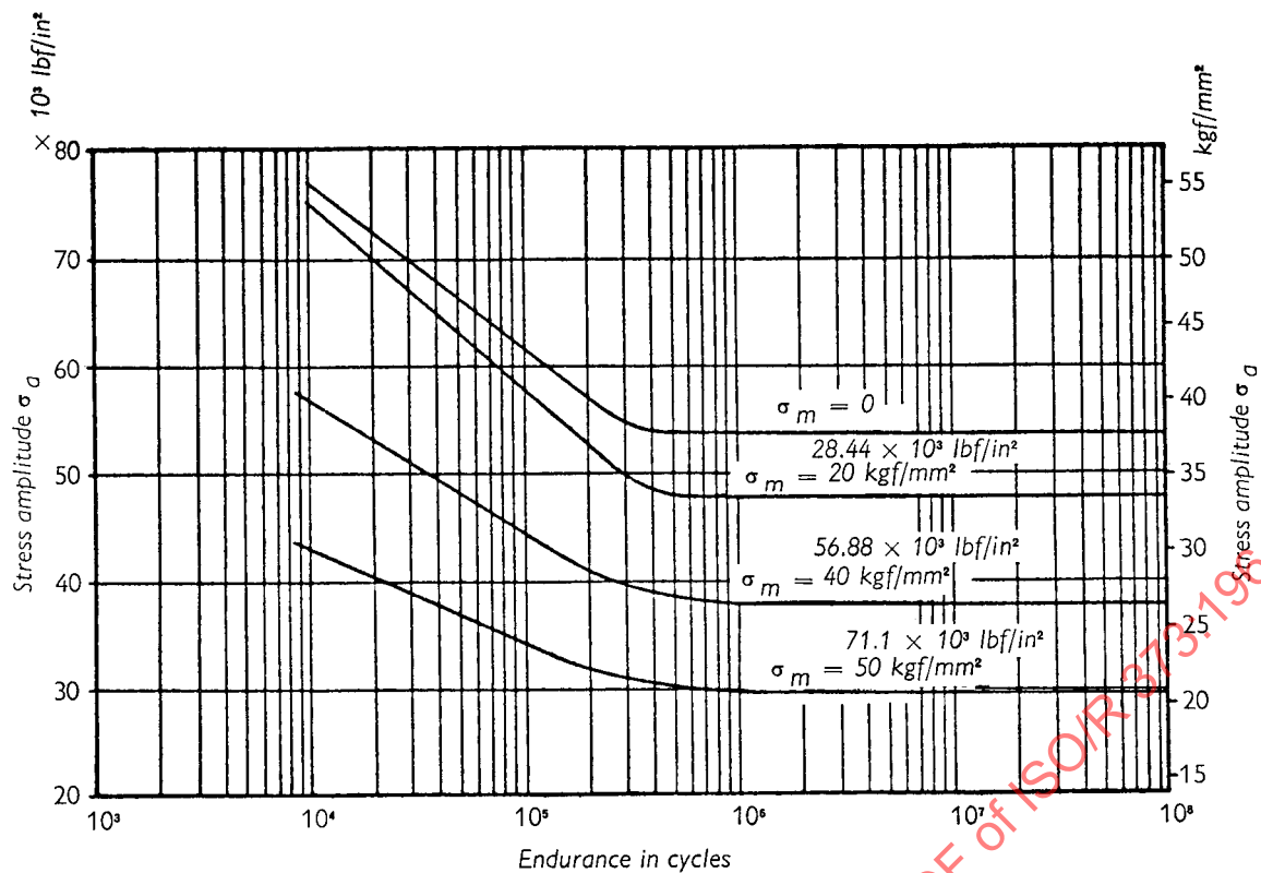
Fig. 6. — S/N curves corresponding to particular mean stresses (linear stress scale)
