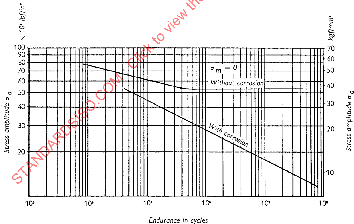
Fig. 5. — S/N curves (logarithmic stress scale)
