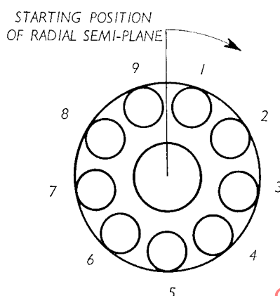
FIG. 4. — Numbering of turbine engine combustion chambers
