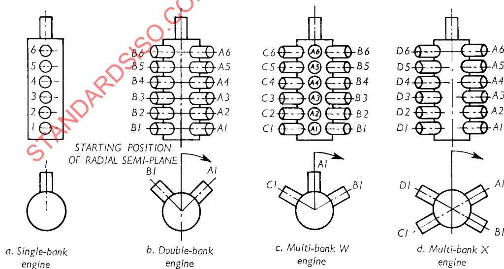
FIG. 2. — Numbering of cylinders of in-line piston engines
