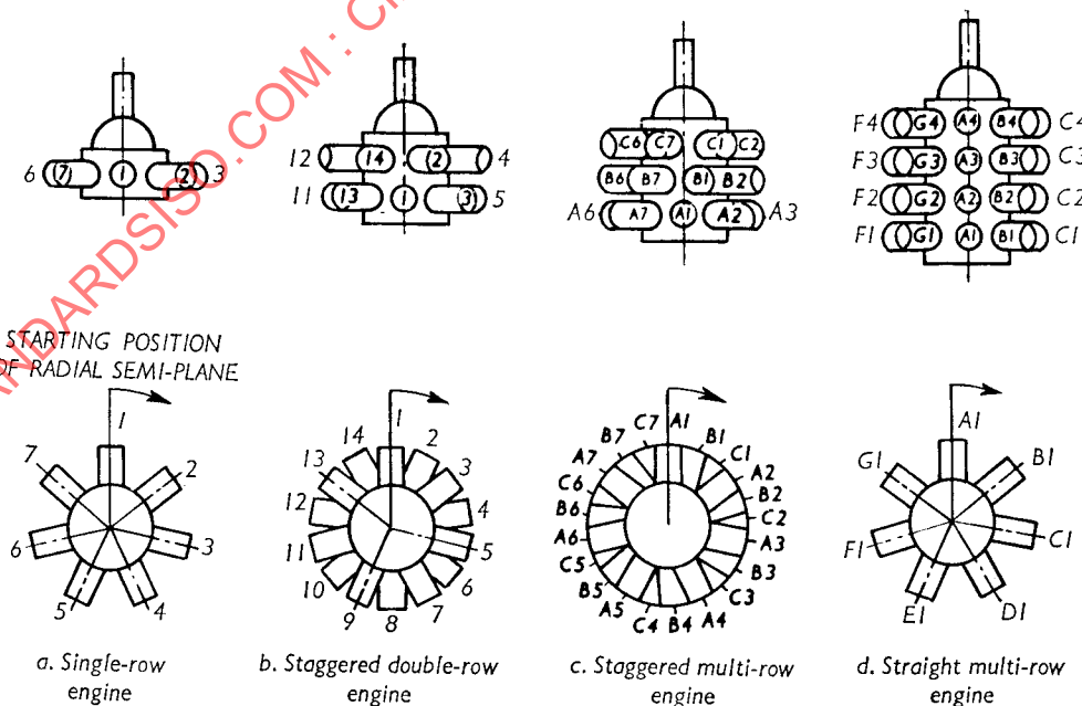
FIG. 3. — Numbering of cylinders of radial piston engines
