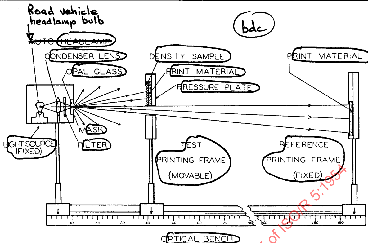
Fig. 6 — Apparatus for Contact Printing Method
