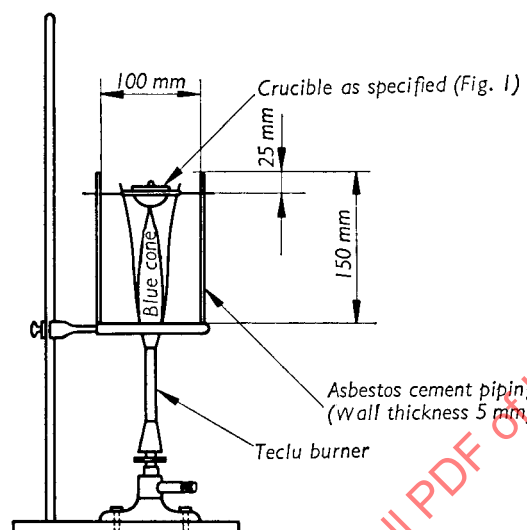
FIG. 3. — Apparatus for the gas heating method
