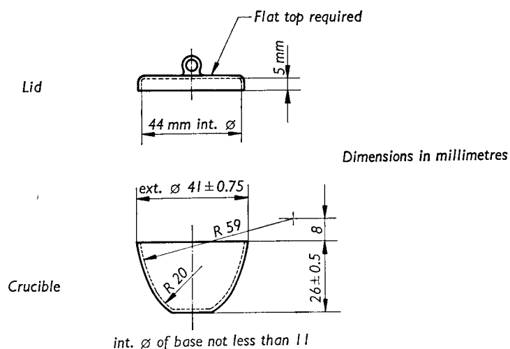
FIG. 1. — Crucible with lid for swelling test
