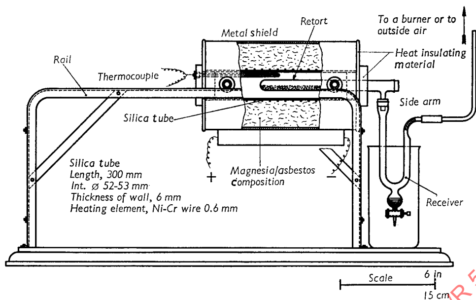
FIG. 2. — Single tube furnace
