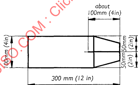
FIG. 3. — Tapered test piece
