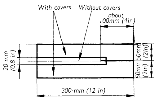
FIG. 1. — Test piece with breaker
