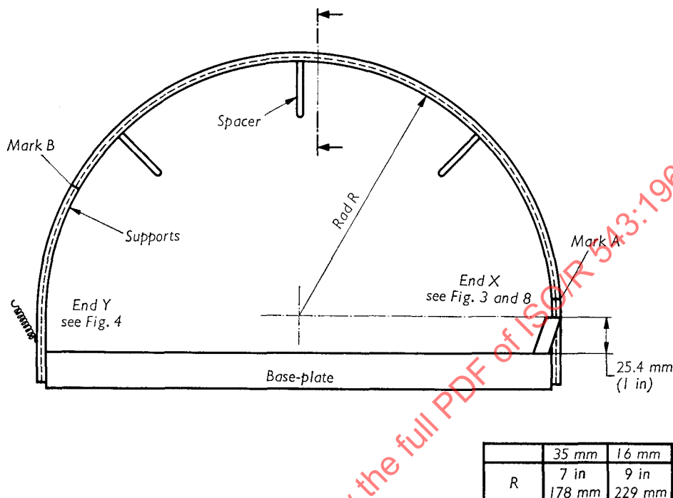
FIG. 1. — General arrangement of apparatus for flammability test of safety film
