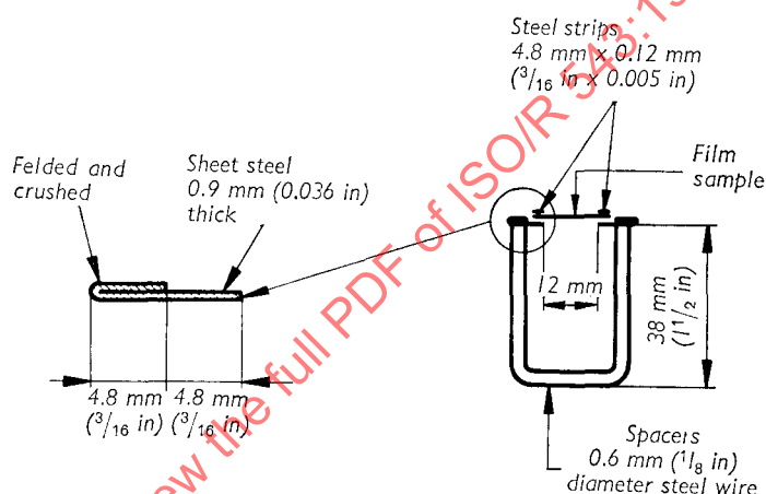
FIG. 7. — Section through supports, showing wire spacers for 16 mm film apparatus
