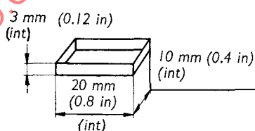
FIG. 5. — Alcohol cup for 35 mm film apparatus
