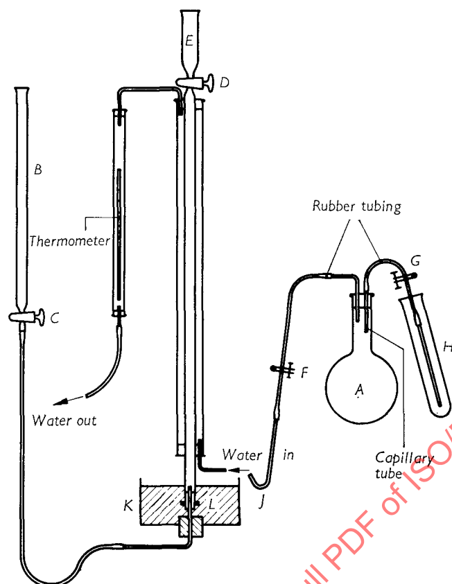
FIG. 8. — Schulze-Tiemann method for determination of nitrate nitrogen content
