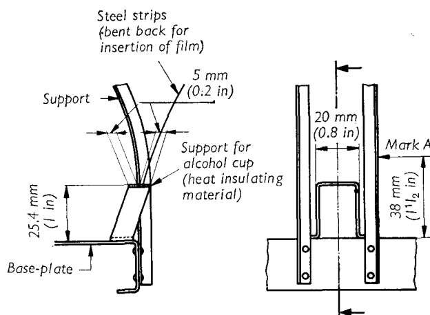
FIG. 3. — Detail of end X for 35 mm film apparatus
