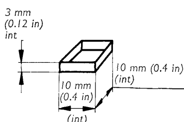
FIG. 6. — Alcohol cup for 16 mm film apparatus
