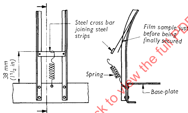
FIG. 4. — Detail of end Y for 35 mm film apparatus
