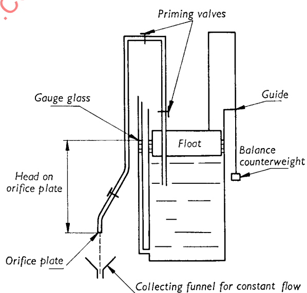
FIG. 6. — Floating siphon for injecting concentrated solution
