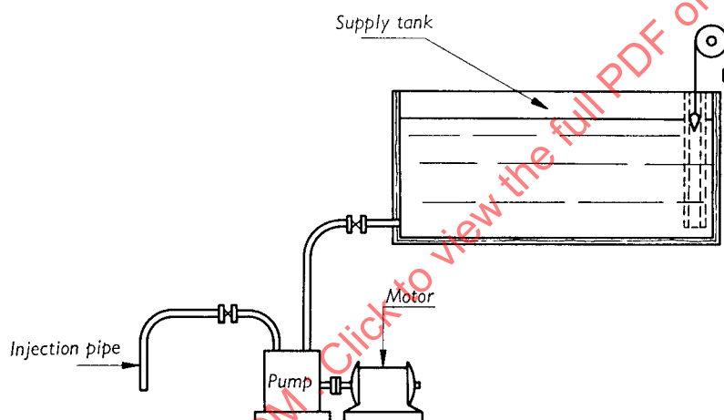
FIG. 4. — Arrangement for injecting concentrated solution by rotary volumetric pump
